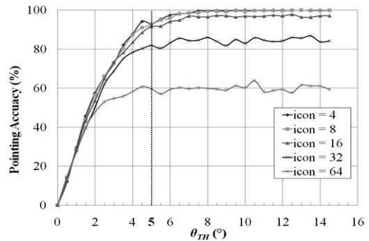
Fig.6. Pointing accuracy with the number of virtual icons and \theta_{TH}
