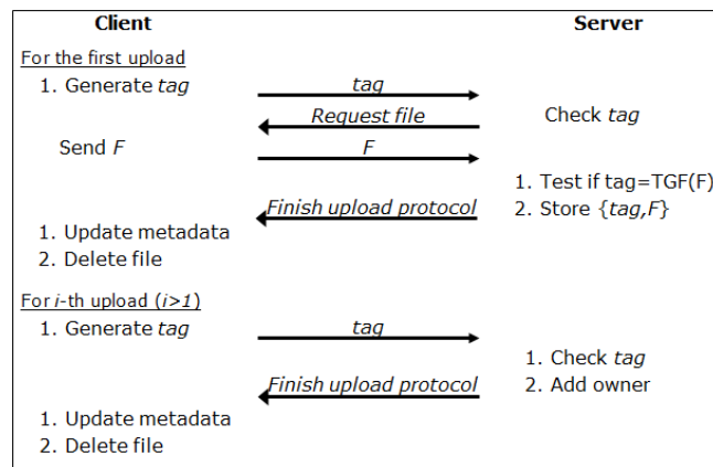
Figure 3. Naive deduplication.
