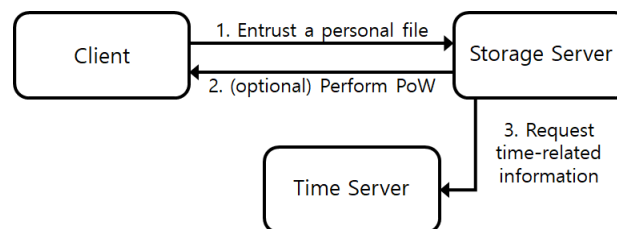
Figure 2. Time-based Locked Deduplication System.
