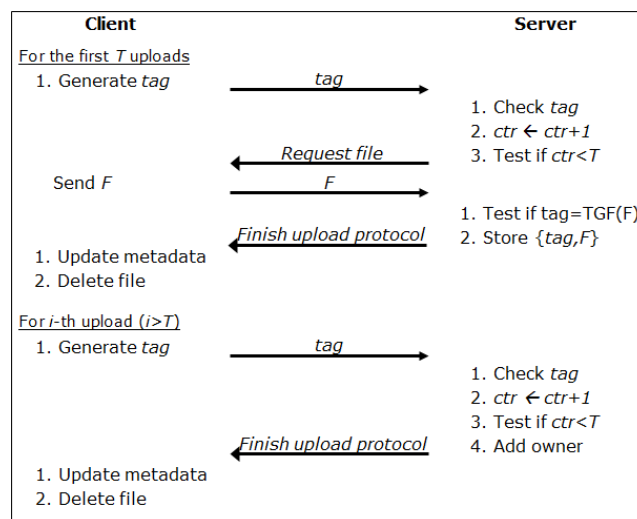
Figure 4. Counter-based client-side deduplication.
