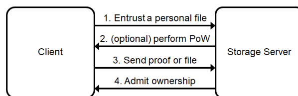
Figure 1. Client-side deduplication.
