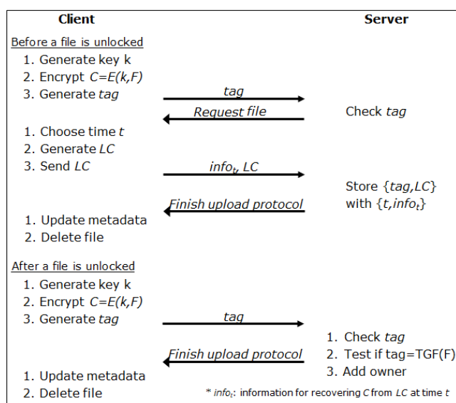
Figure 5. Time-locked deduplication (Basic Construction).
